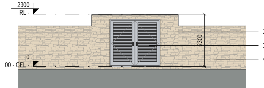
2 Front Elevation 1:100
