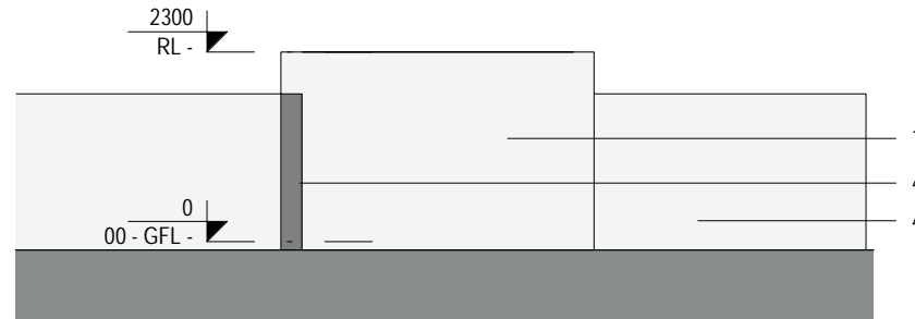
7 Rear Elevation 1:100
