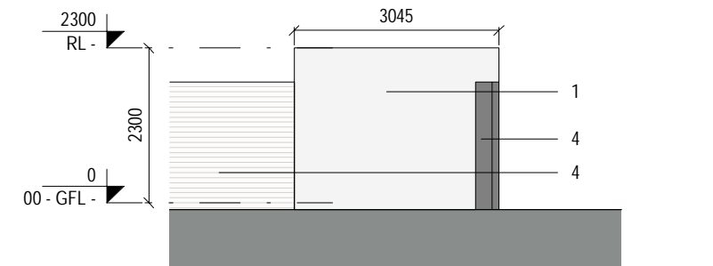
6 Side Elevation B 1:100
